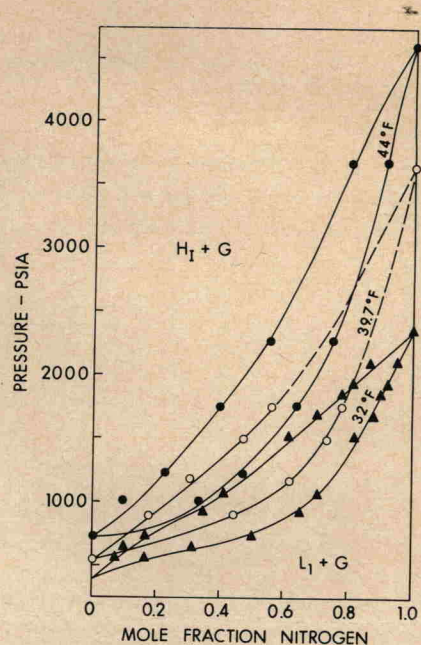
Figure 2—Pressure composition diagrams for the nitrogen-methane-water system.
